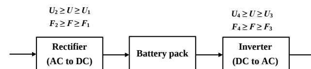
Figure 1 – Example of an AC power source design
