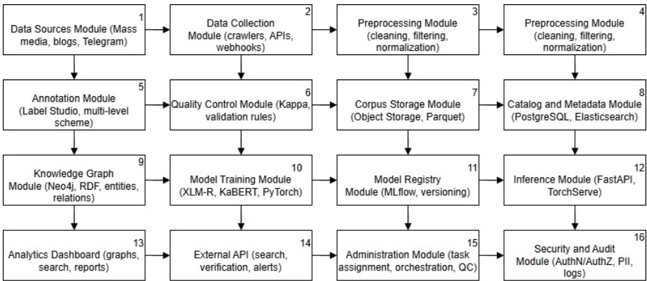
Figure 3 – The architecture of the adaptive model of detection of fake news
