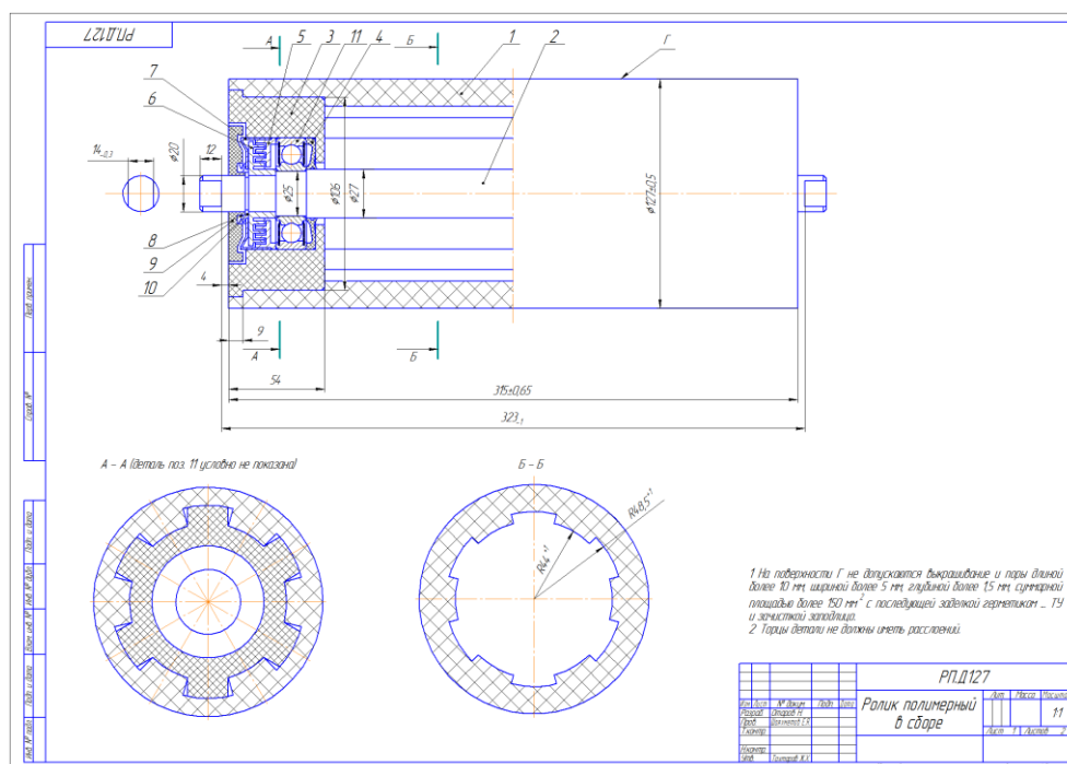
Figure 1 – Roller made of polymer materials in assembly
