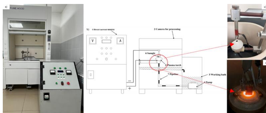
Figure 1 – Electrolytic-plasma treatment unit and diagram
